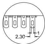
Solder eyelet Type
